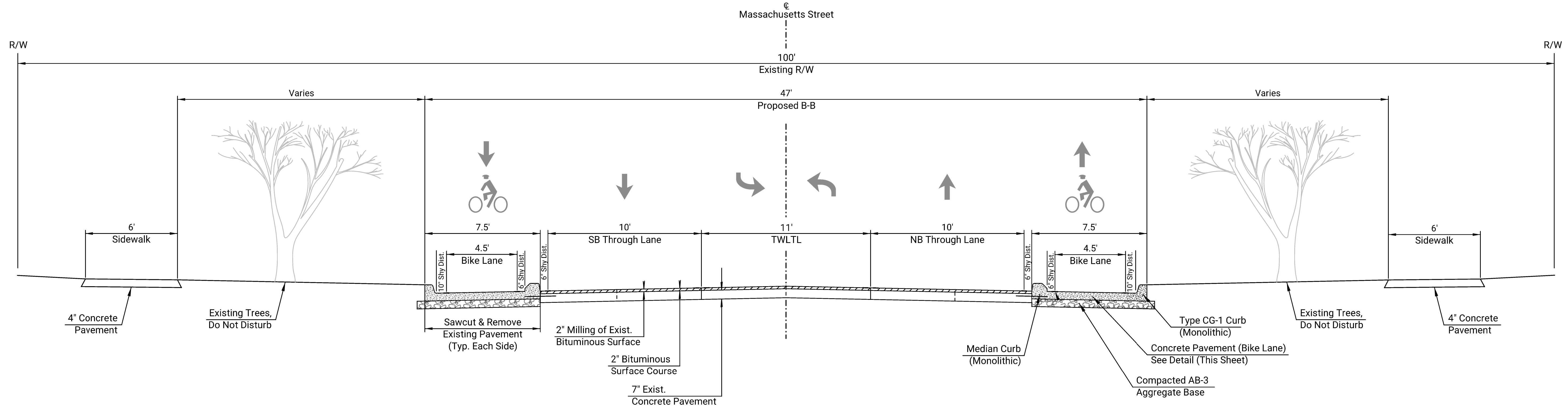
Typical Section Massachusetts Street 14th St to 23rd St
