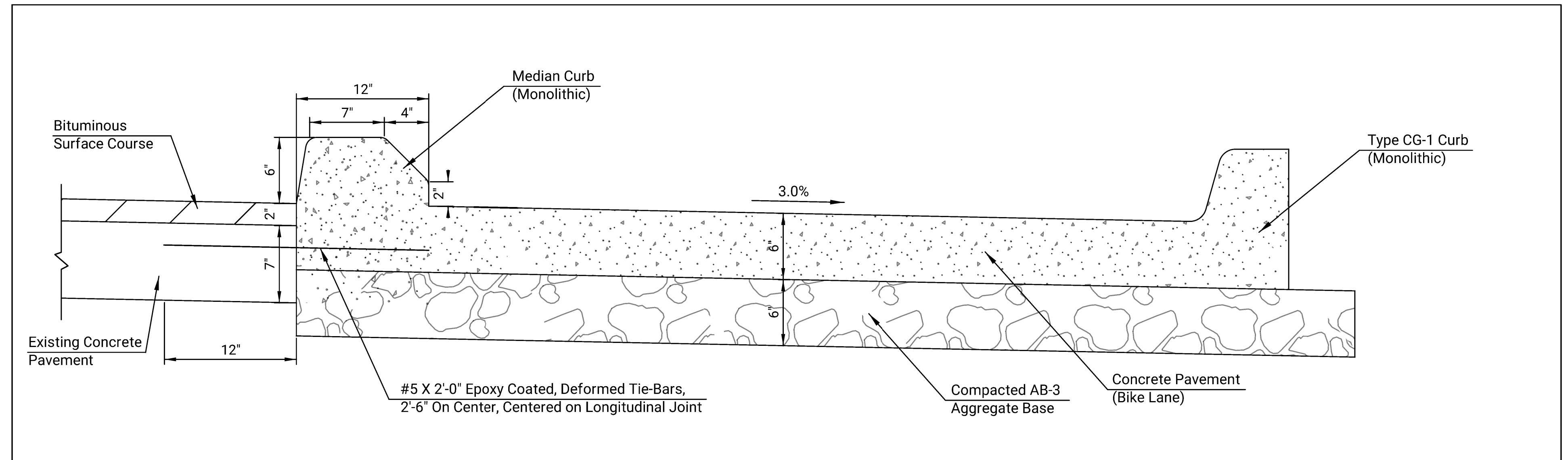
Concrete Bike Lane Detail (Not to Scale)
